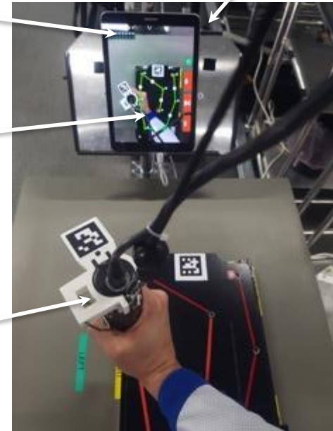
Server algorithm for tracking power tool usage and screw insertion, remotely over 5G.
